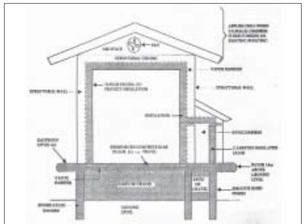
6.4. Design for conditioned seed store
